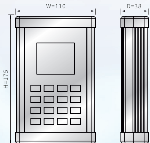
Transmitter Dimensions (Unit: mm)
