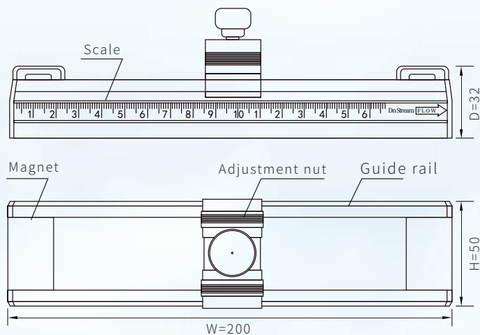
Transducer Dimensions(Unit: mm)
