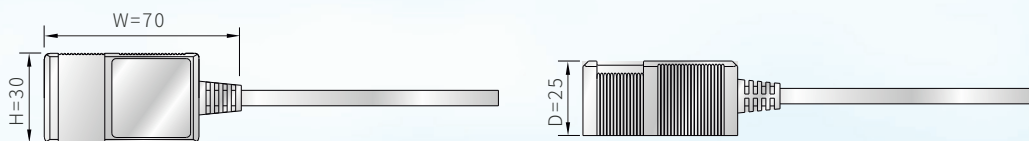
Transducer Dimensions(Unit: mm)
